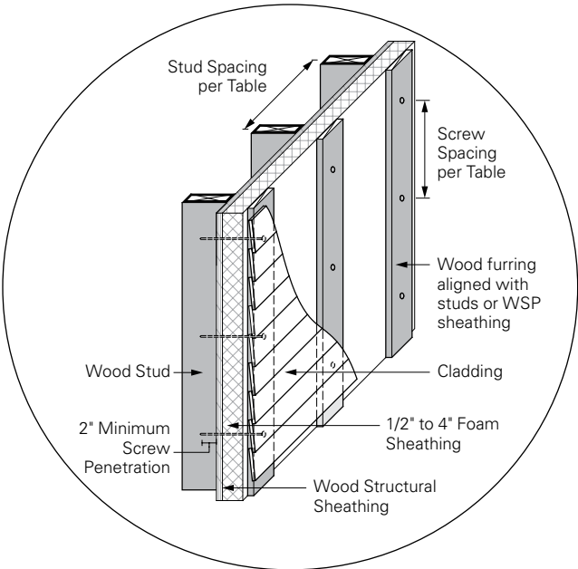
Figure 1—Cladding Over Foam Sheathing
